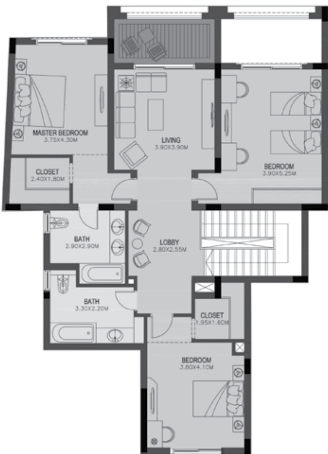
BEDROOMS LEVEL PLAN
